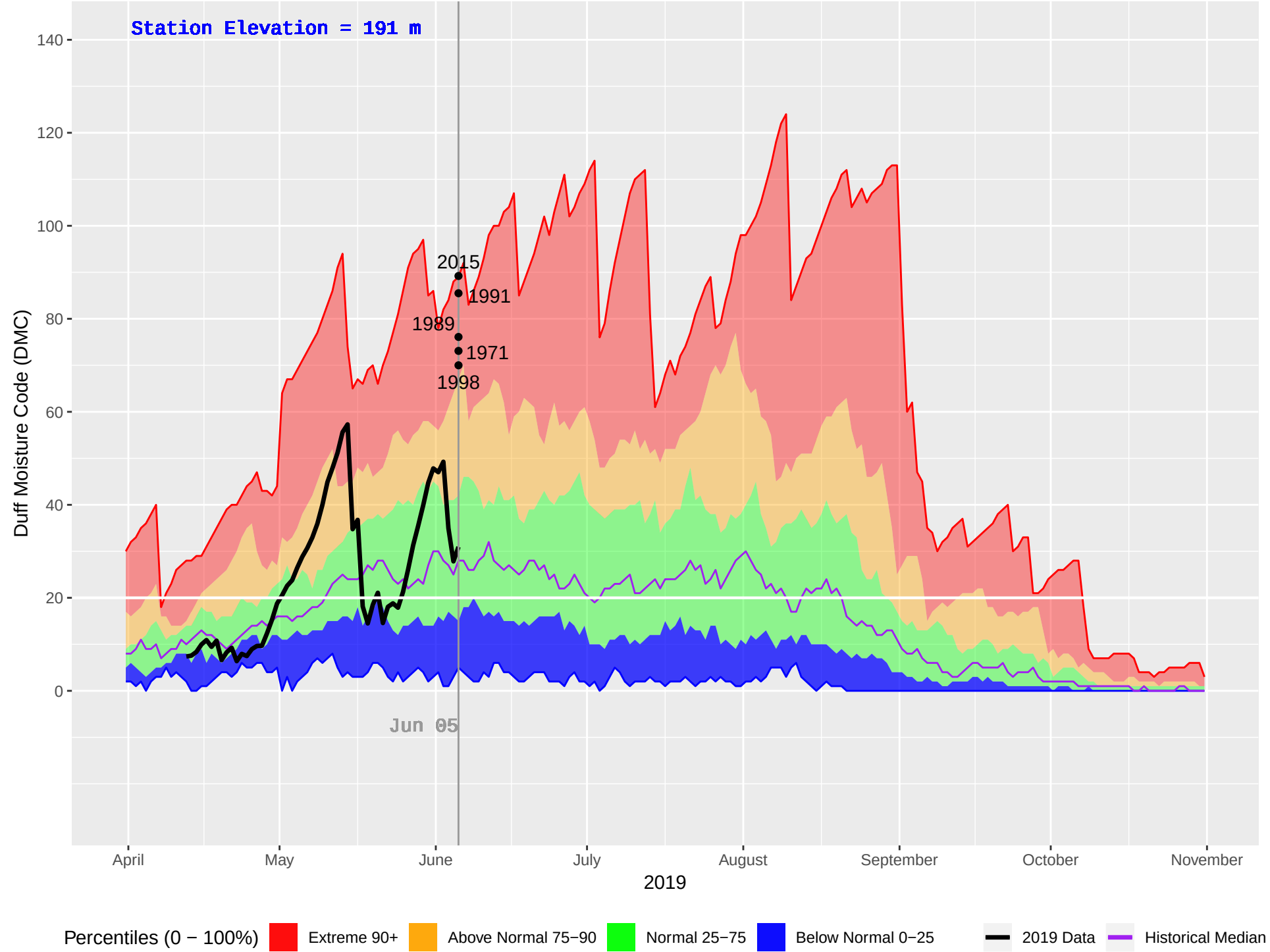
NASS CAMP (427) : Historical (1970–2018), Current (2019) Daily Duff Moisture Code (DMC)
