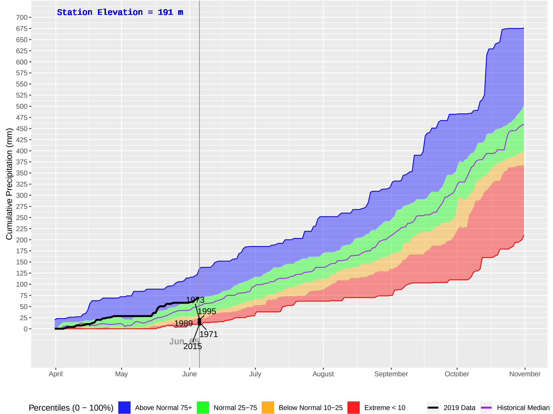
NASS CAMP (427) : Historical (1970–2018), Current (2019) Daily Cumulative Precipitation
