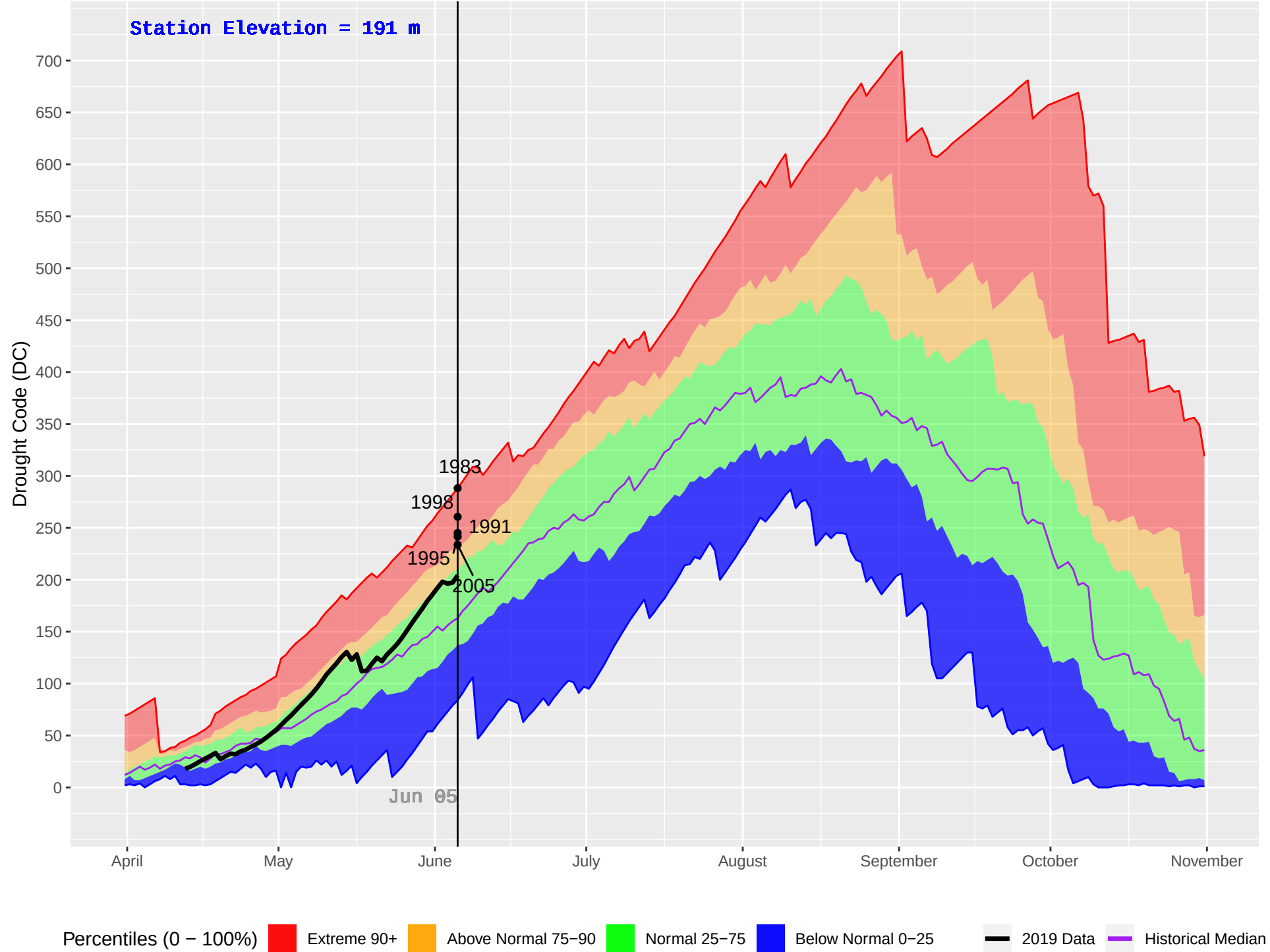
NASS CAMP (427) : Historical (1970–2018) and Current (2019) Daily Drought Code (DC)
