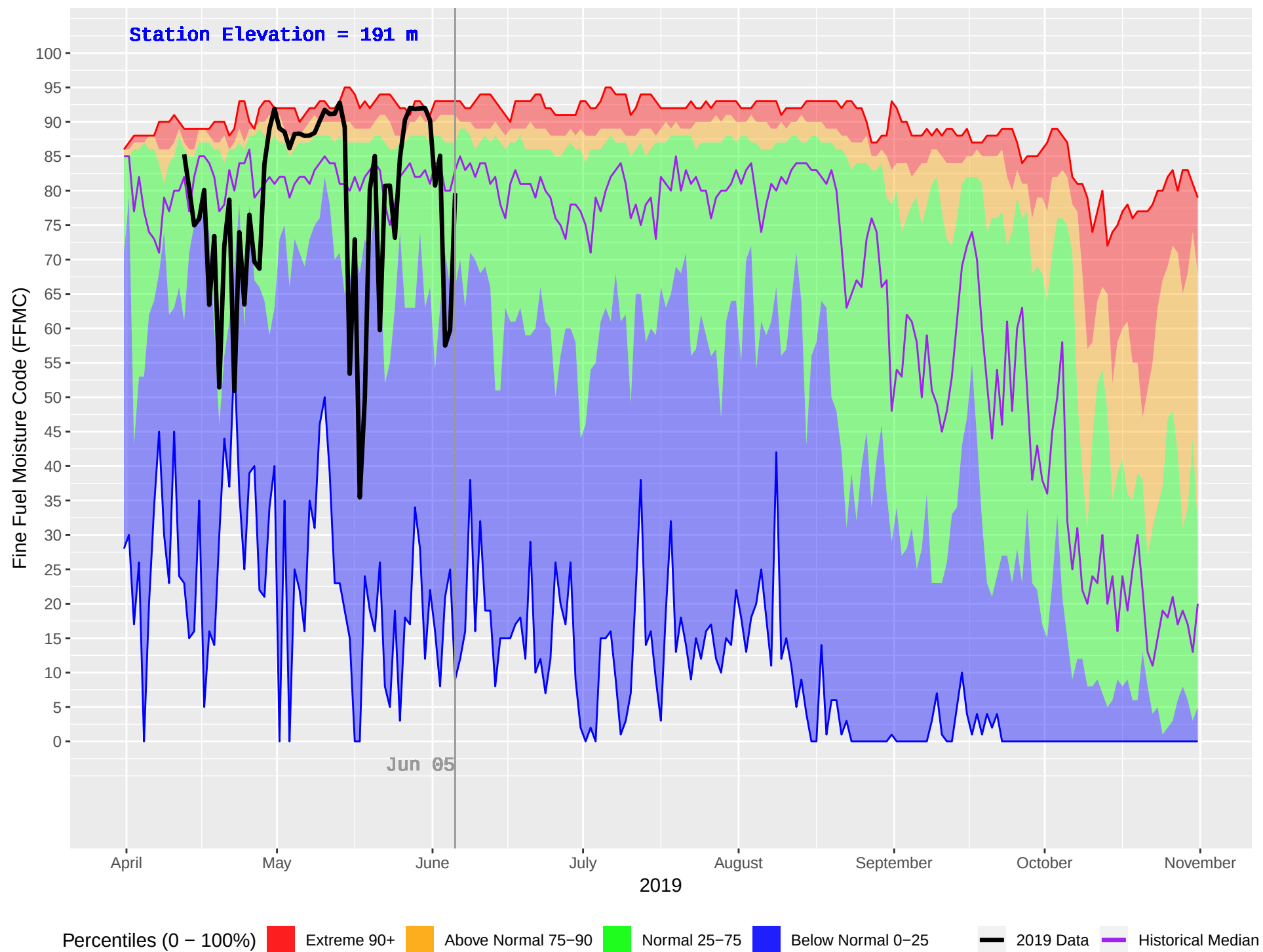
NASS CAMP (427) : Historical (1970–2018) and Current (2019) Daily Fine Fuel Moisture Code (FFMC)
