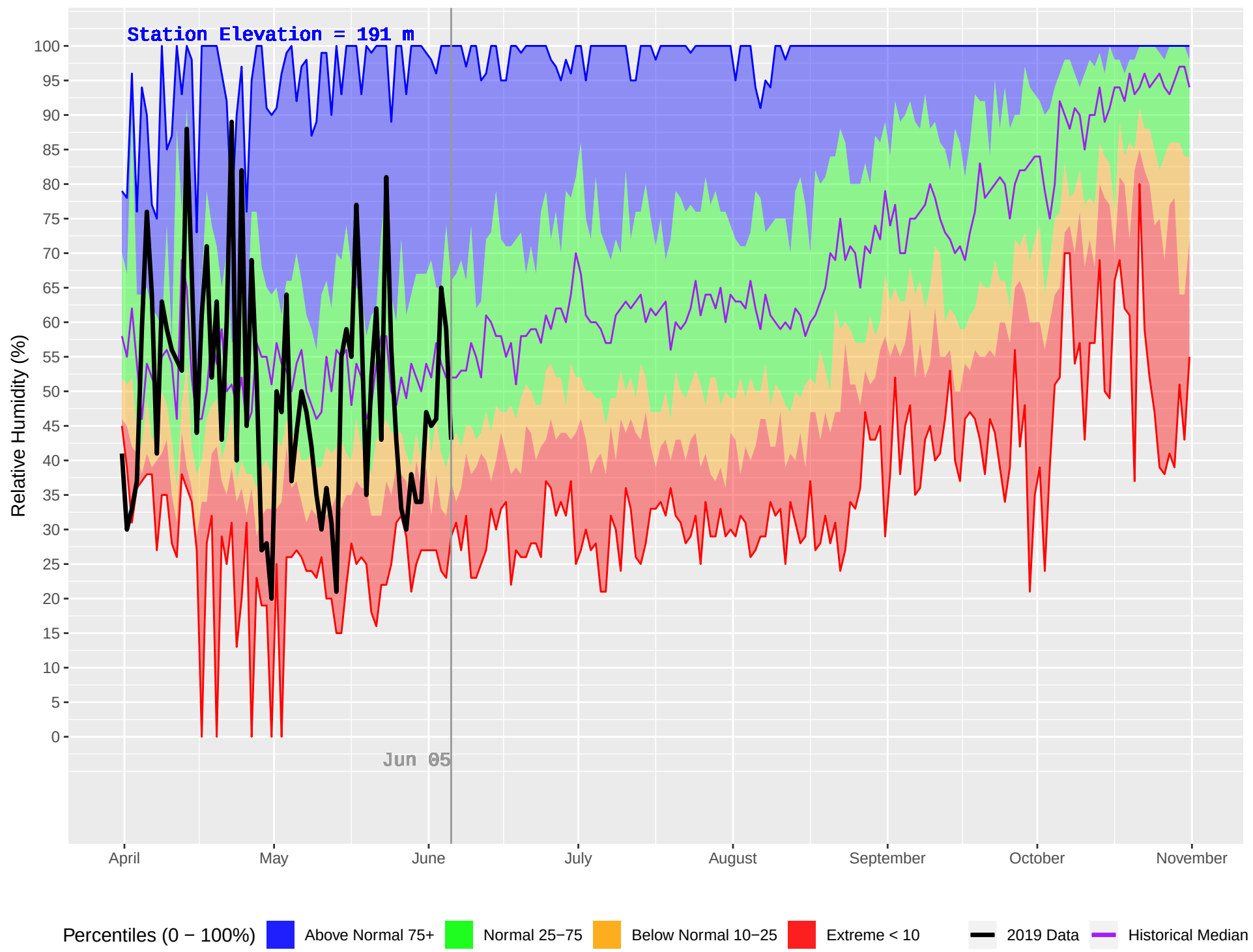
NASS CAMP (427) : Historical (1970–2018) and Current (2019) Daily Relative Humidity
