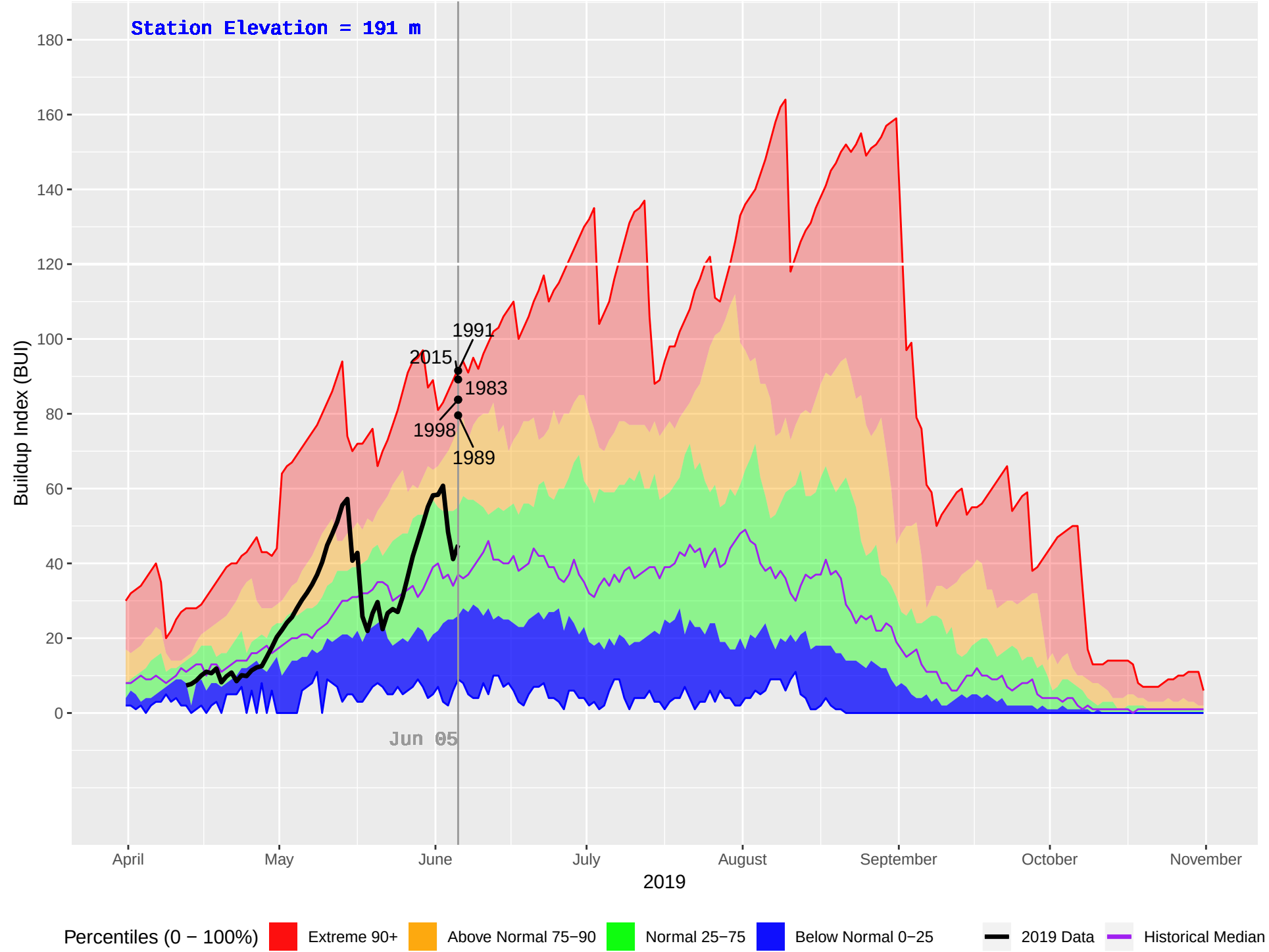
NASS CAMP (427) : Historical (1970–2018), Current (2019) Daily Buildup Index (BUI)
